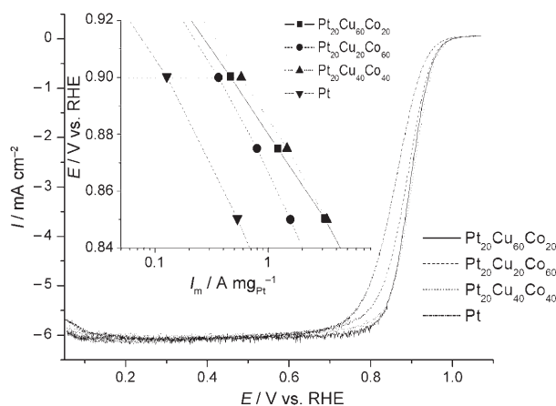
Figure 2. Oxygen reduction reaction (ORR) activity measurements of Pt–Cu–Co ternary alloy nanoparticle catalysts in an RDE setup. Inset: Pt-mass-based activities ( \text{A}_{\text{mgPt}}^{-1} ) over a range of electrode potentials for which the surface catalysis is rate-determining (kinetically controlled region).
